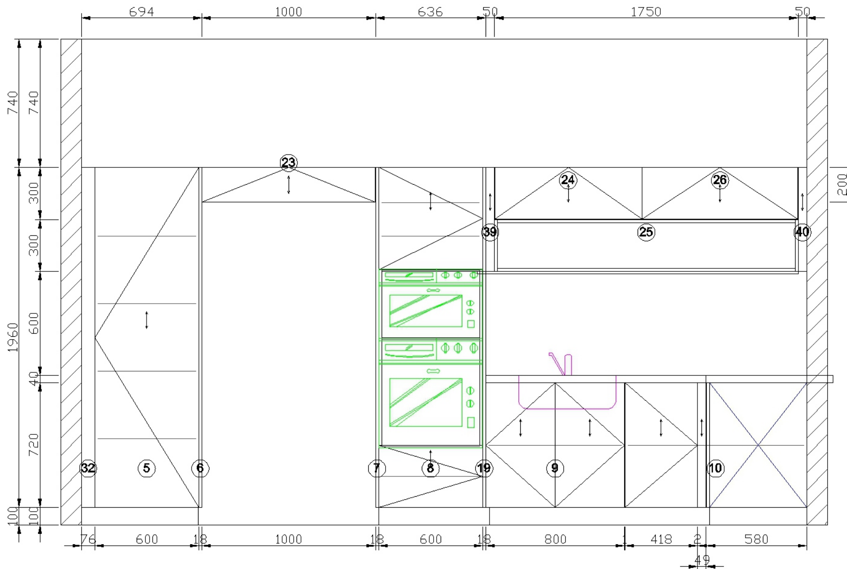
D View elevation drawing
