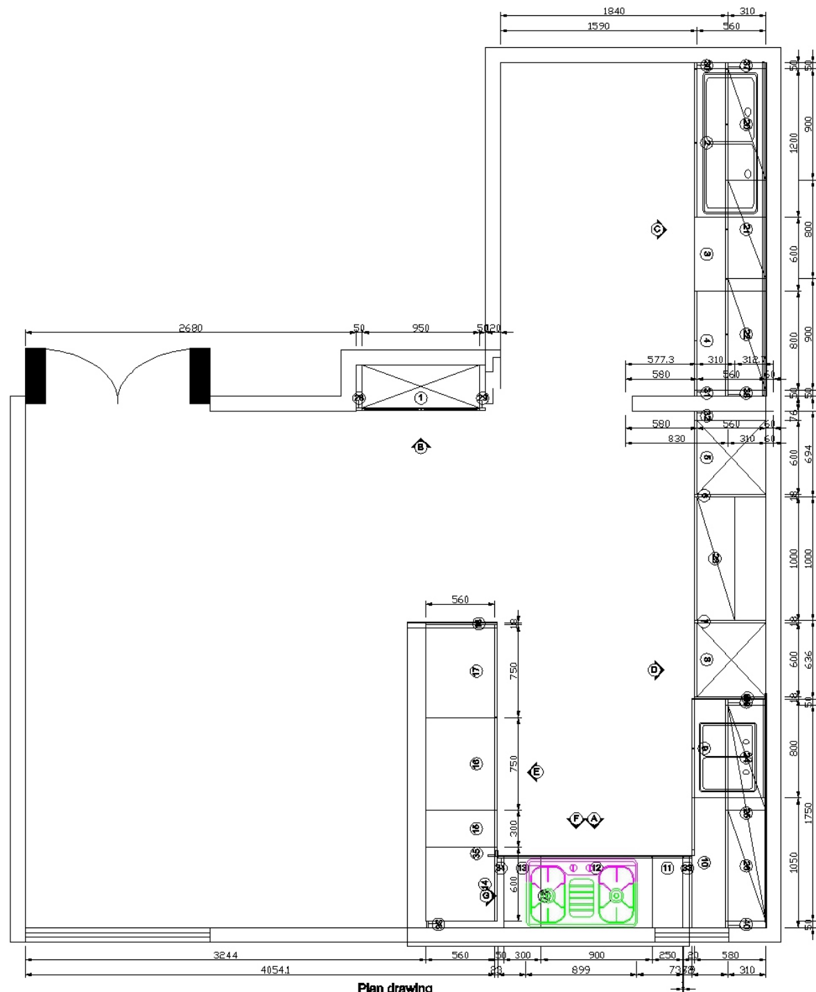
Plan drawing
