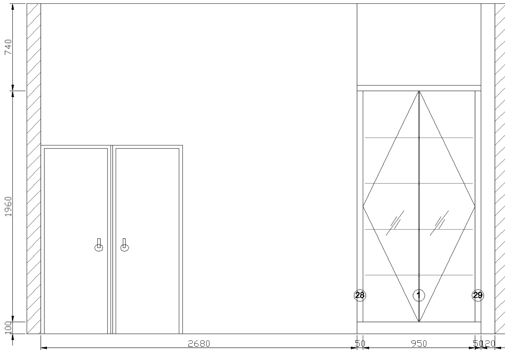
B View elevation drawing
